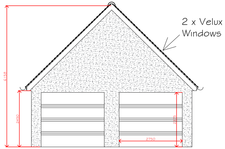
Proposed Front Elevation (Garage)
