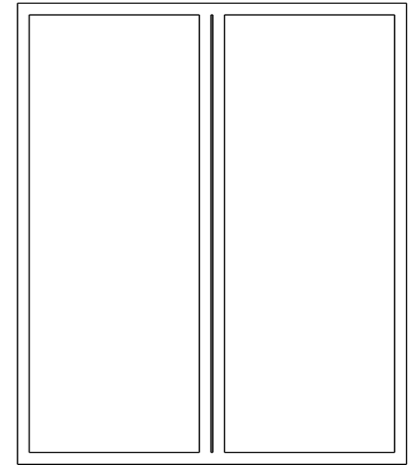
ID11 - 1810x2150mm Double Glazed with Internal Shutters Wooden Frame Painted Blue external side?
